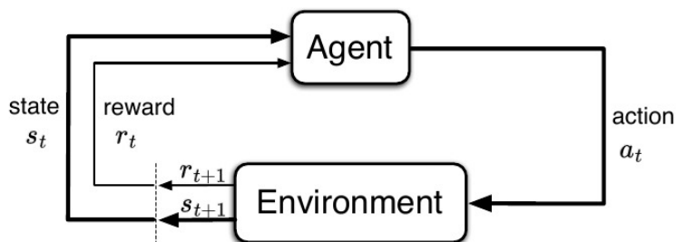
Figure 2: Diagram of the reinforcement learning interaction between the agent and its environment, from Sutton and Barto (2018).
