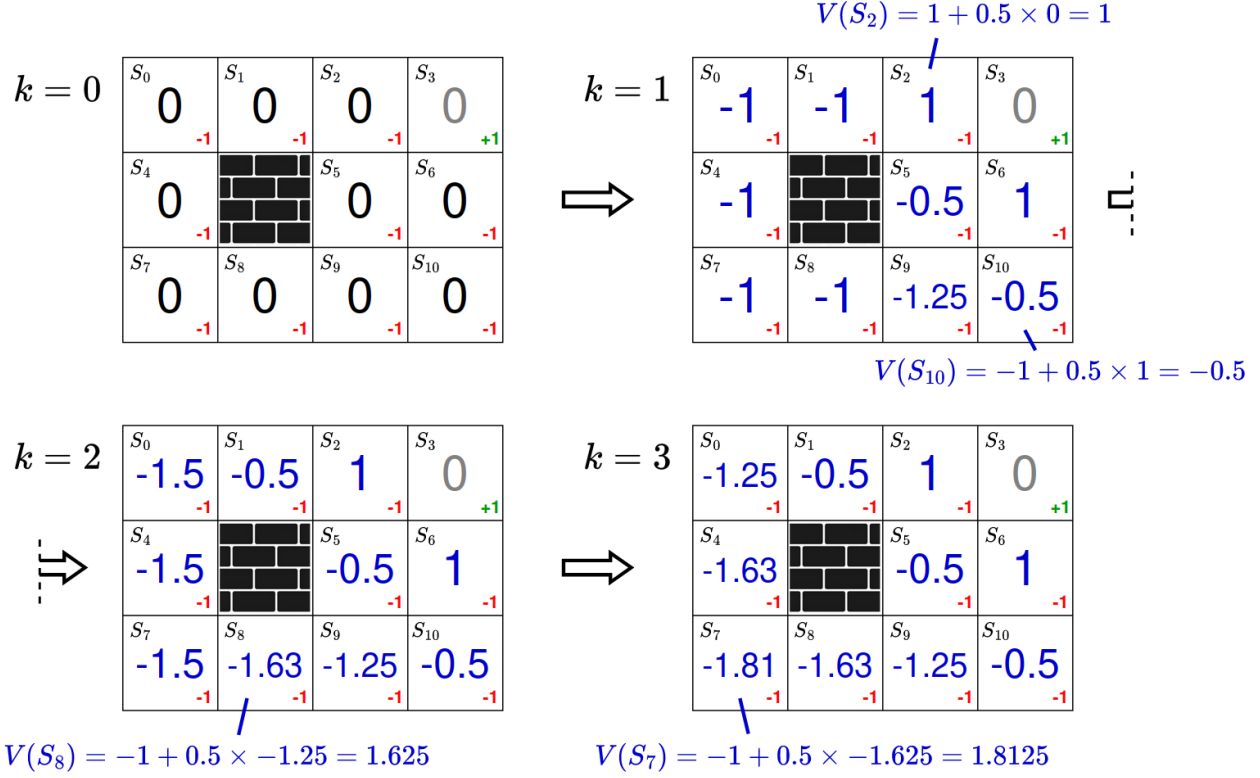
Figure 4: Value iteration algorithm executed on the example of Figure 3. We start with an initial value function V(s) = 0 for all s \in \mathbf{S} . Then, each iteration k applies the update rule of Equation 15, with \gamma = 0.5 , with the result V(s_t) shown in the corresponding cell. As state s_3 is terminal, its value is considered to be 0. In three iterations, we converge to the optimal value function. Note that, because we compute the new V for each state successively, the order of the states affects the result of each iteration and the number of iterations required for converging.
