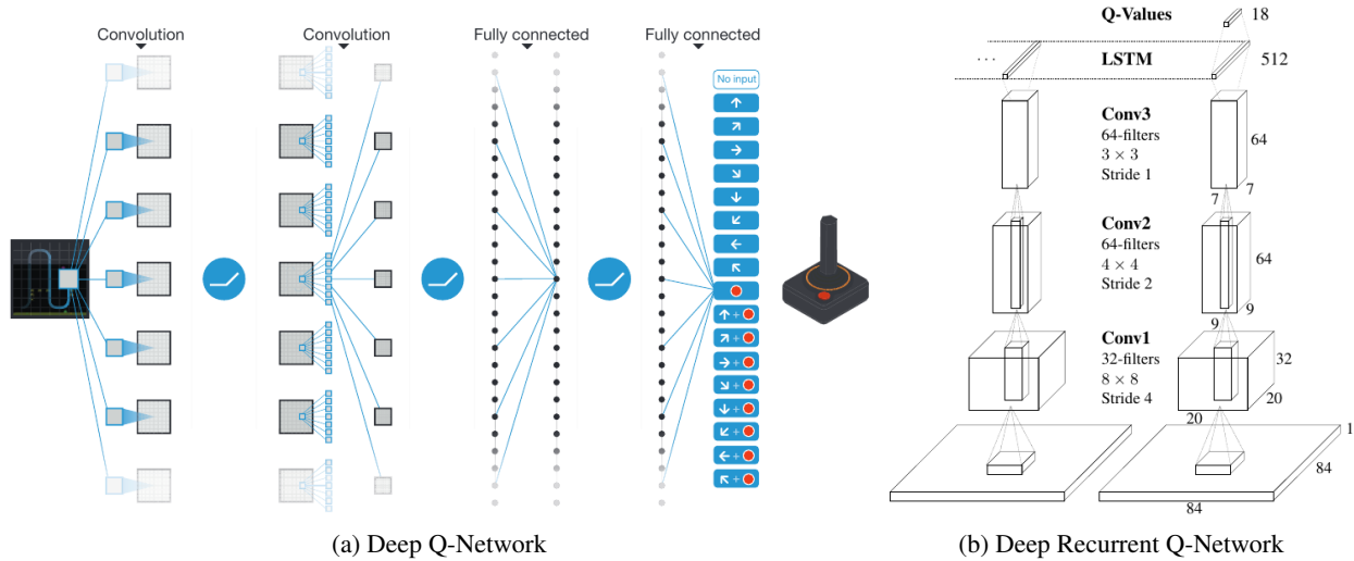
Figure 5: DQN architectures. (a) The original DQN (Mnih et al., 2015), with a series of convolution layers that analyse the input frame, followed by fully connected layers that output the value of each action. (b) Recurrent version of a DQN (Hausknecht & Stone, 2015), that adds an LSTM unit after the convolutions to allow some information to carry to future steps.
